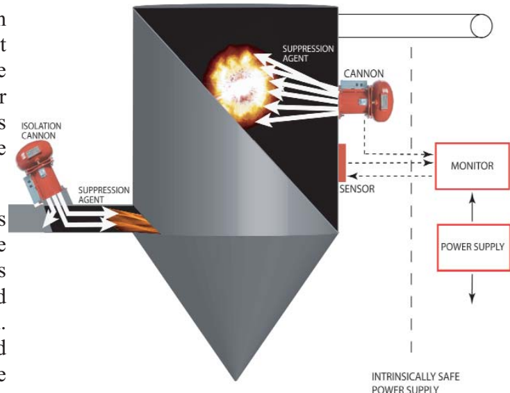
IPD System applied to Dust Collector
